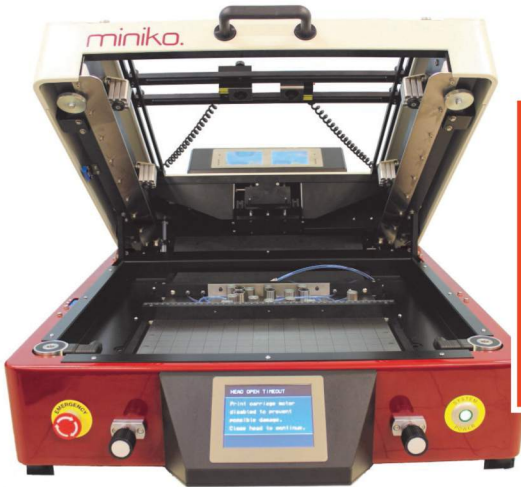
Print head in open position showing easy access to printing table
